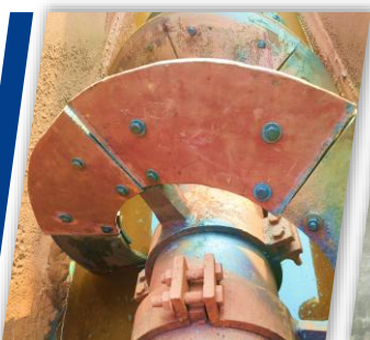
Classifier Liner
